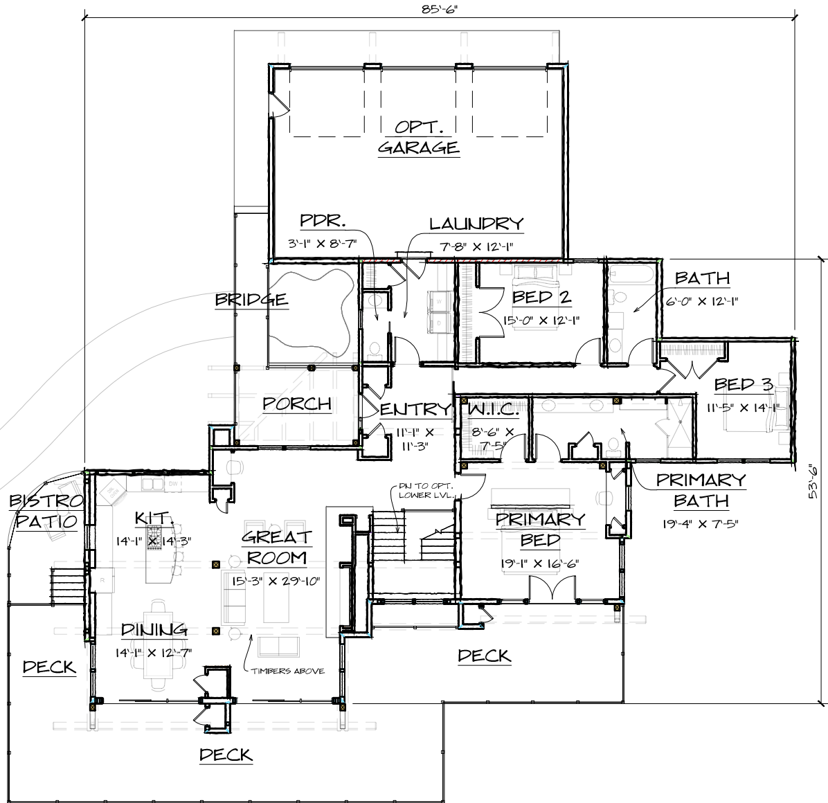
FIRST FLOOR - 2649 SQ. FT.
